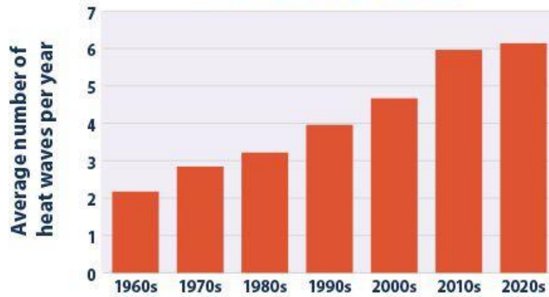
Heat Wave Frequency
