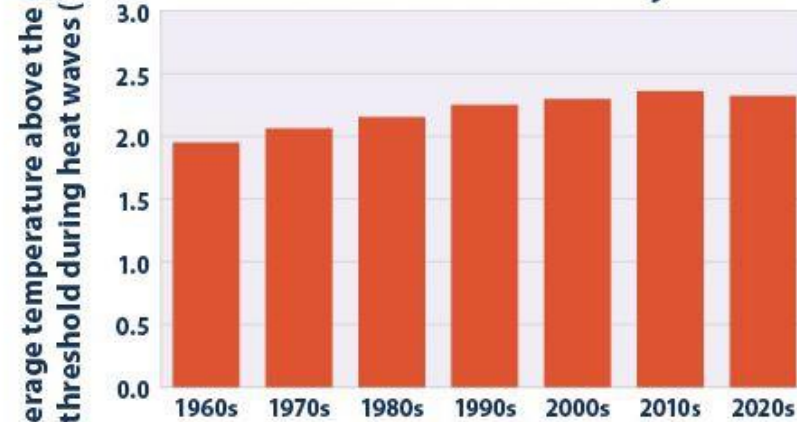
Heat Wave Intensity
